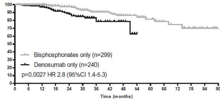
(B) Time-to-ONJ (%):
